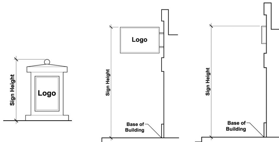
FIGURE 14-2: SIGN HEIGHT
