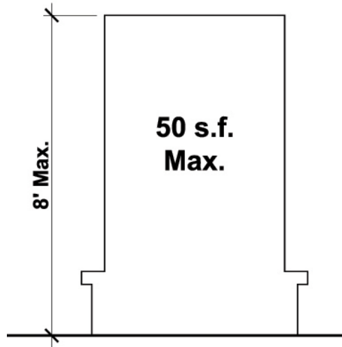
FIGURE 14-5: MONUMENT SIGNS
