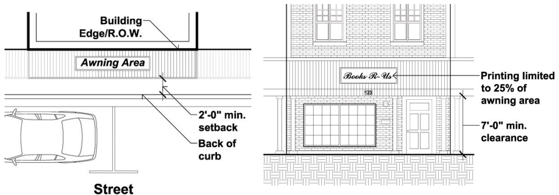
FIGURE 14-4: AWNING SIGNS
