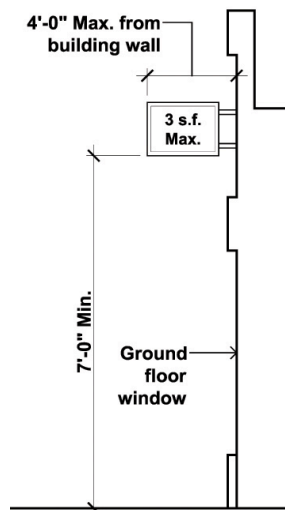
FIGURE 14-7: PROJECTING SIGN
