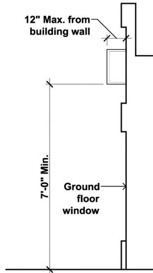
FIGURE 14-8: WALL SIGN
