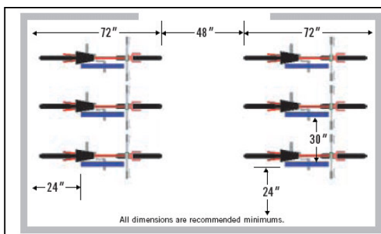
Figure 5-17 Recommended Minimum Dimensions for Bicycle Rack Parking (Source: www.bicyclinginfo.org )
