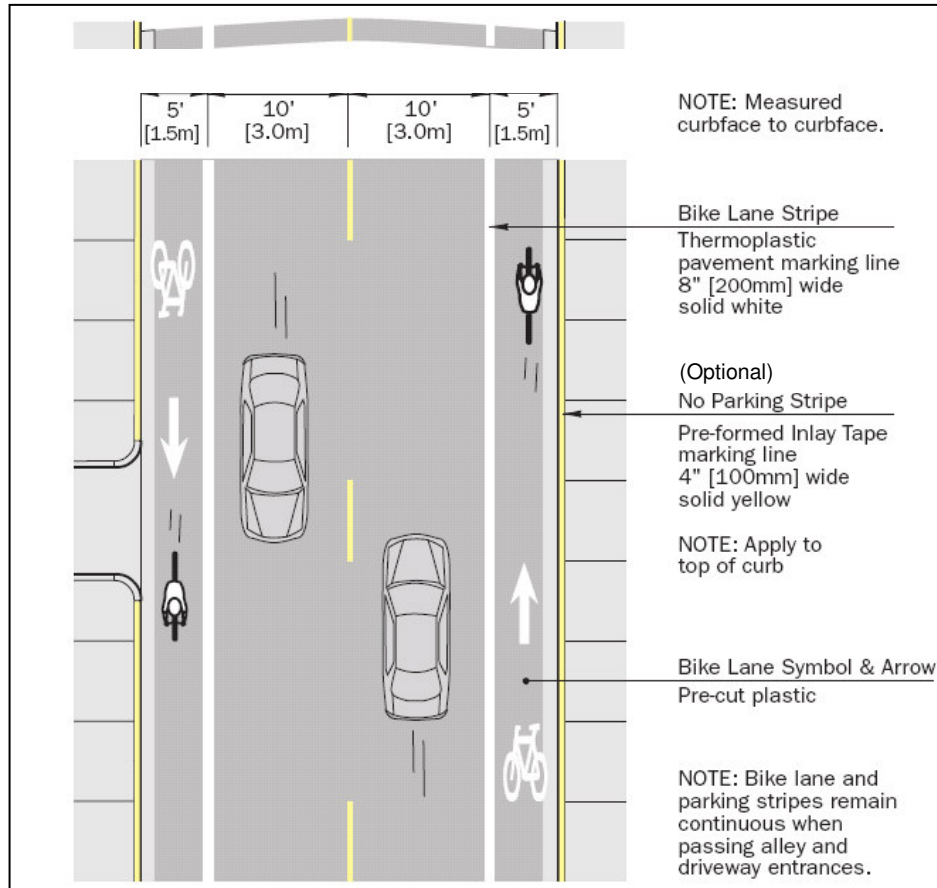
Figure 5-5 Bike Lanes on a 30-foot Wide Street Without On-Street Parking (Source: City of Chicago, Bike Lane Design Guide)
