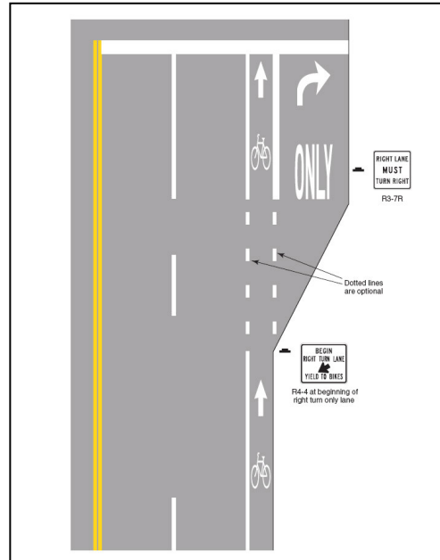
Figure 5-8: Bicycle Lane Treatment at Right Turn Only Lane (Source: MUTCD 2003)
