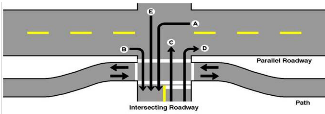
Figure 5-2 Shared Use Path/Roadway Intersection (Source: AASHTO)
