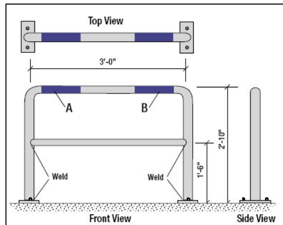
Figure 5-16 Inverted "U" Bicycle Rack (Source: www.bicyclinginfo.org )
