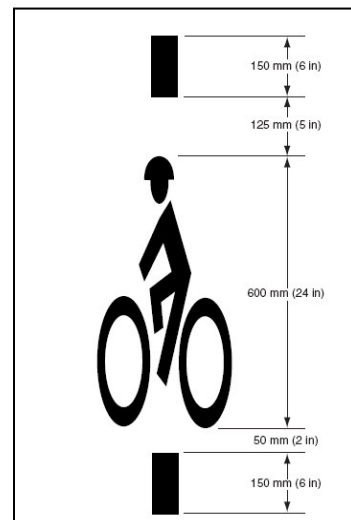
Figure 5-15 Bicycle Detector Pavement Marking (Source: MUTCD 2003)
