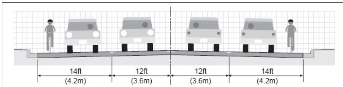
Figure 5-13 Wide Outside Lanes (Source: Wisconsin Bicycle Facility Design Handbook)
