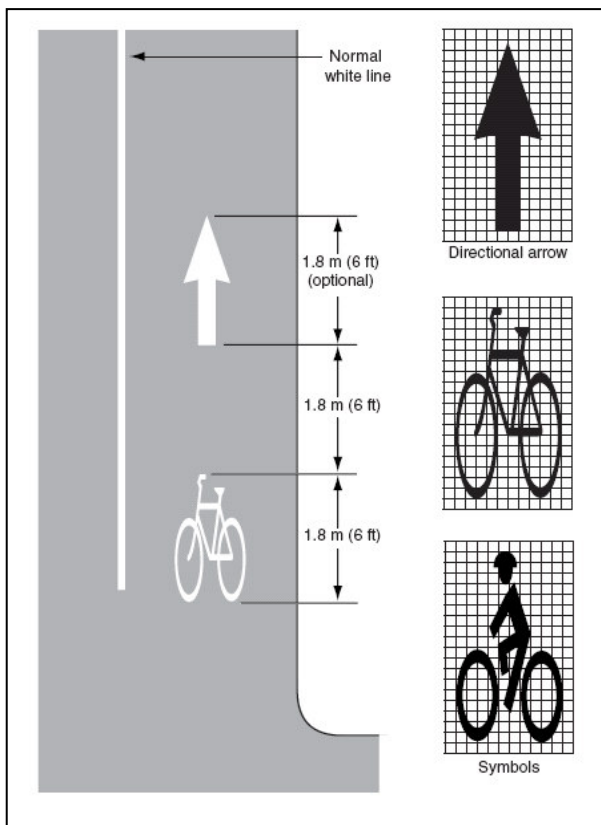
Figure 5-6: Optional Symbol Pavement Markings for Bike Lanes (Source: MUTCD 2003)
