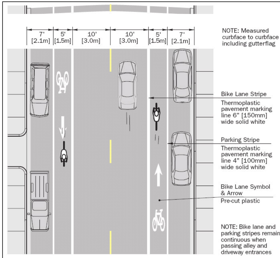
Figure 5-4 Bike Lanes on a Narrow Two-Way Street With On-Street Parking (Source: City of Chicago, Bike Lane Design Guide)
