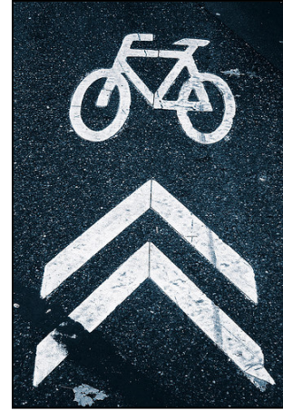
Figure 5.14: Shared Lane Pavement Marking
