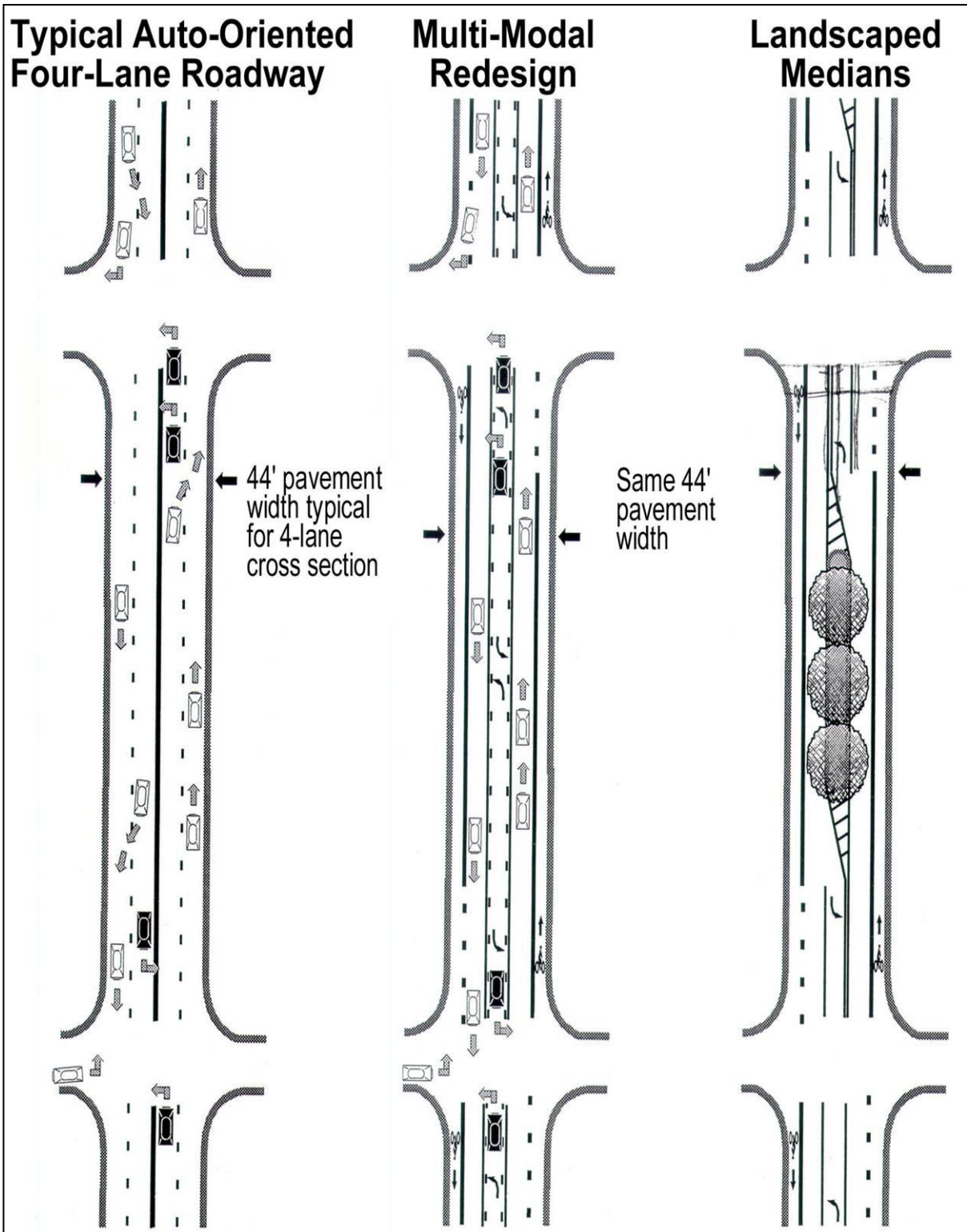
Figure 5-11 Reducing the Number of Vehicular Travel Lanes (Source: Kalamazoo Non-motorized Transportation Plan)
