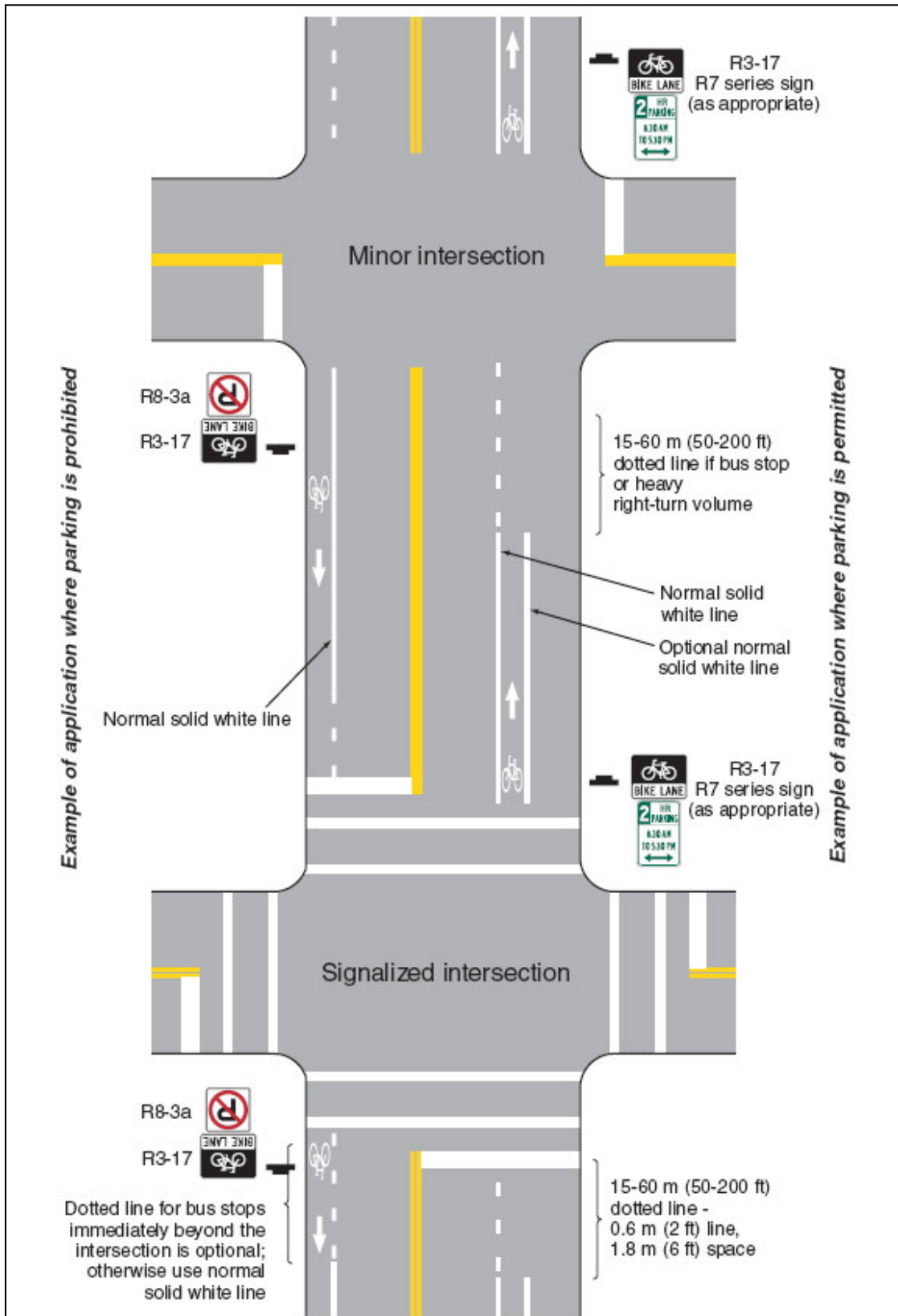
Figure 5-7: Example of Pavement Markings for Bicycle Lanes on a Two-Way Street (Source: MUTCD 2003)
