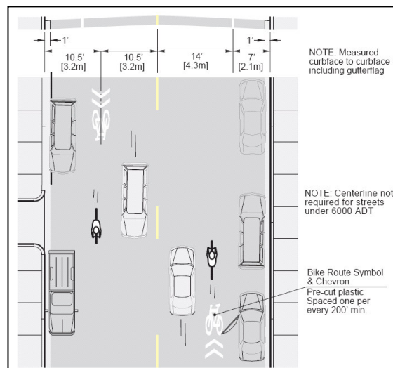
Figure 5-9: Signing of Shared Lanes (Source: MUTCD)
